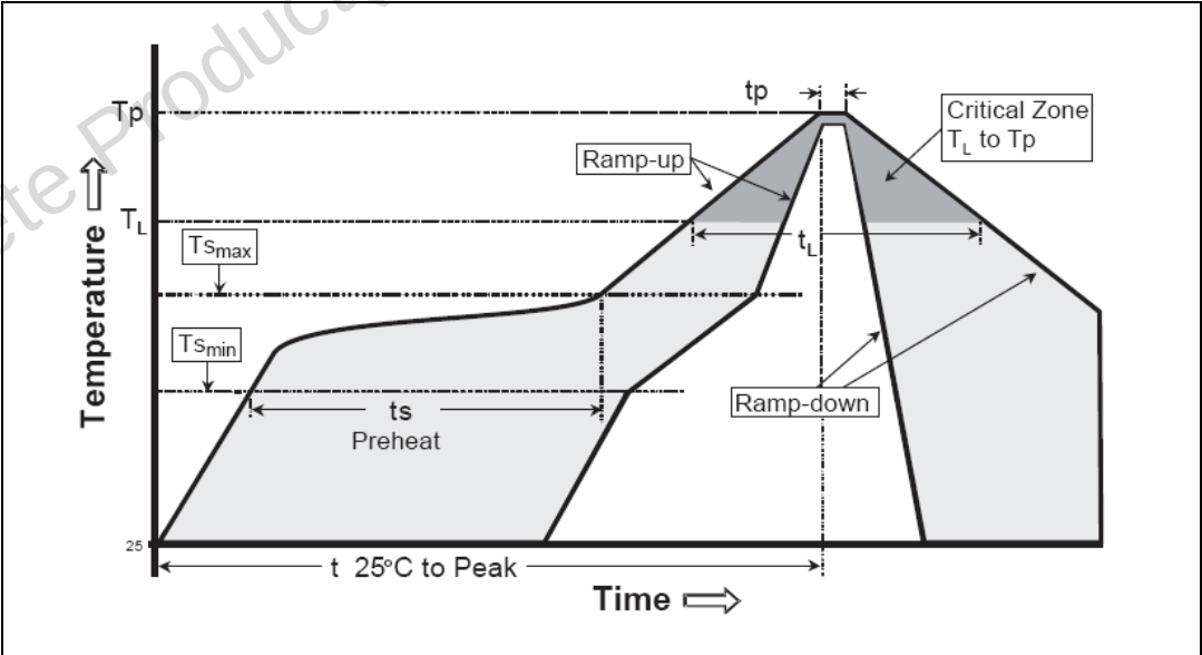
Figure 8. Soldering
